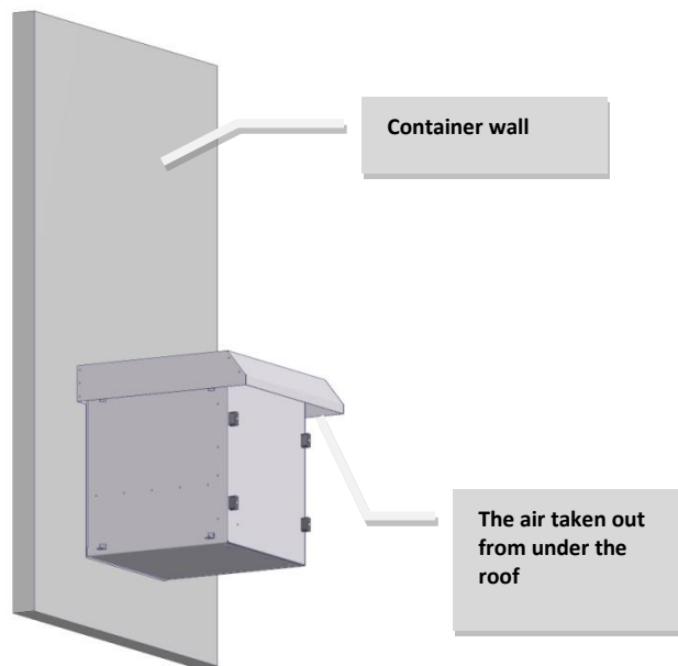
Fig 2. Cool air inlet is located at the bottom of the container
