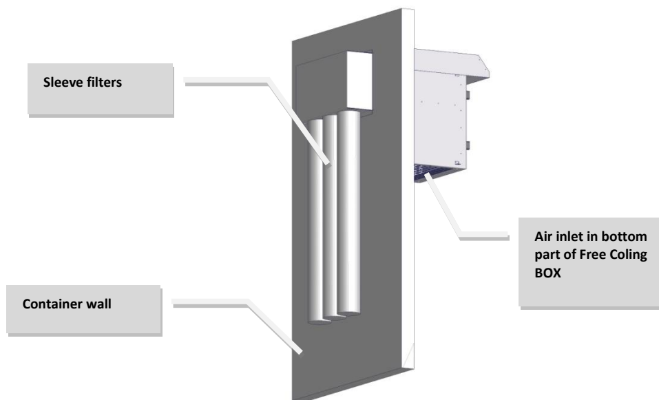
Fig 4. Air inlet in top part of container wall – possibility of using sleeve filters
