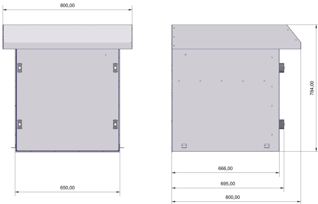
Fig 5. Freecooling Box - dimensions
