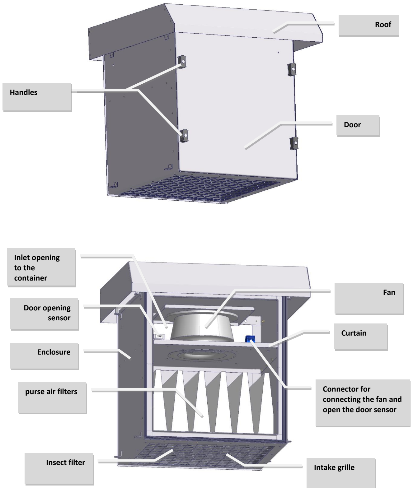
Fig 6. Freecooling BOX
