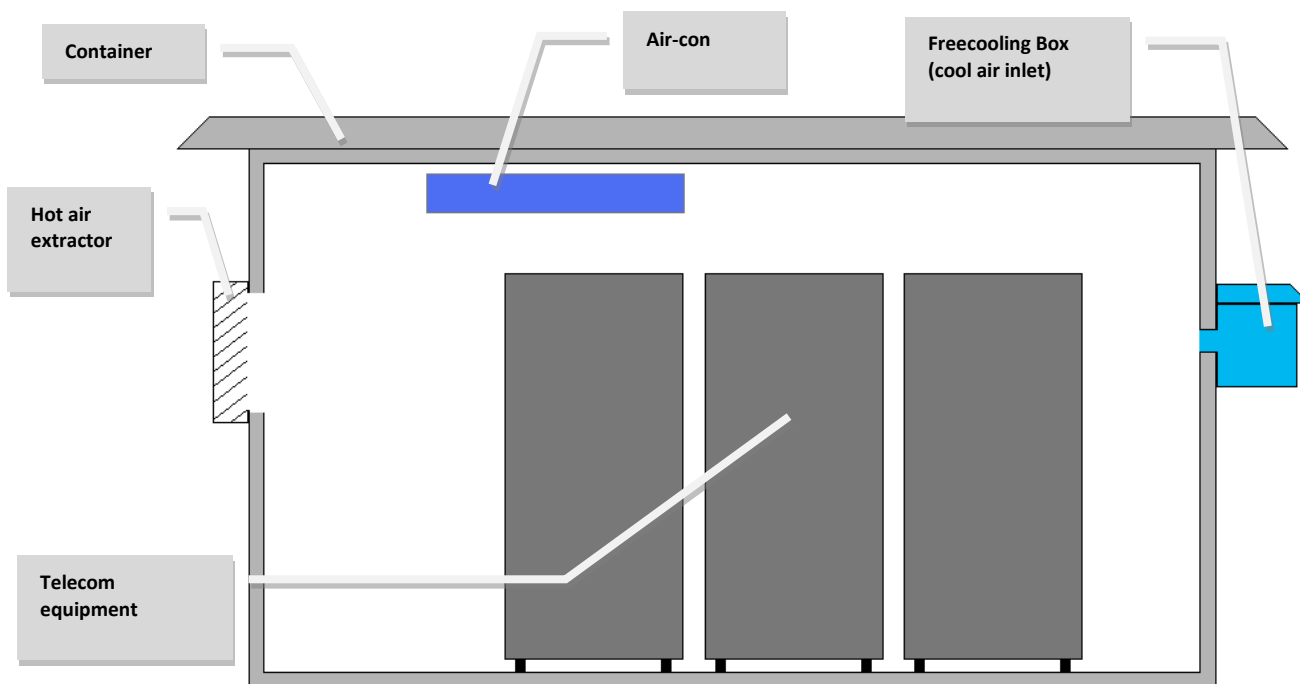
Fig 1. Overview of items layout in a container
