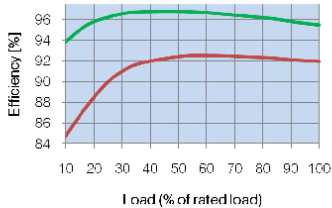
Efficiency Curve: Standard vs High efficiency
